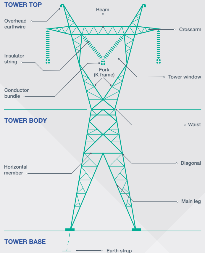
Figure 2: Example transmission tower
