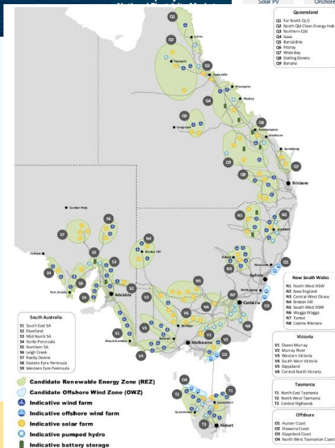
Figure 1.1 Renewable Energy Zone locations in the draft 2022 Integrated System Plan
